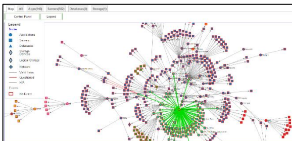
Dependency Analyzer
